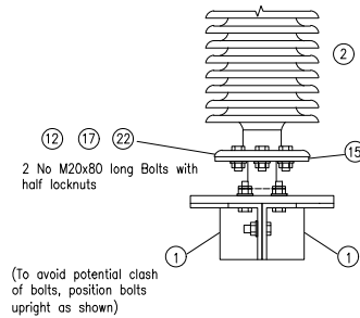
SECTION 2 Scale 1:10
