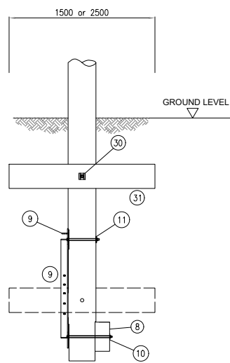
SECTION 4 Scale 1:25
